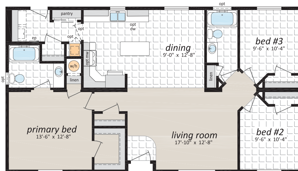
Bedford, 27GL4804 27' x 48' | 1,296 sq. ft. 3 Beds | 2 Baths
