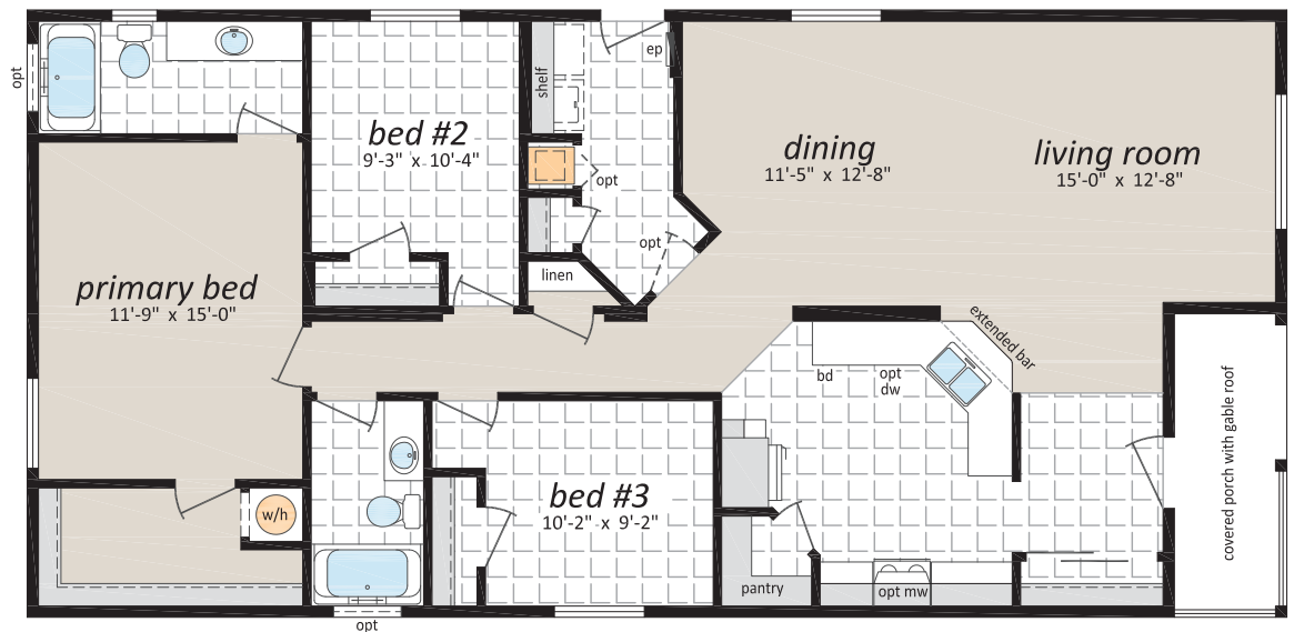
Devon, 27GL5603 27' x 56' 1,512 sq. ft. 3 Beds | 2 Baths
