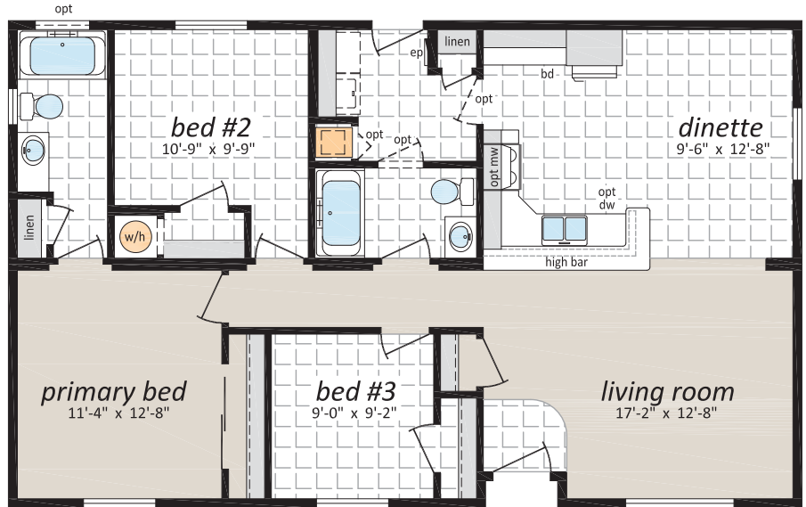
Galiano, 27GL4402 27' x 44' | 1,188 sq. ft. 3 Beds | 2 Baths
