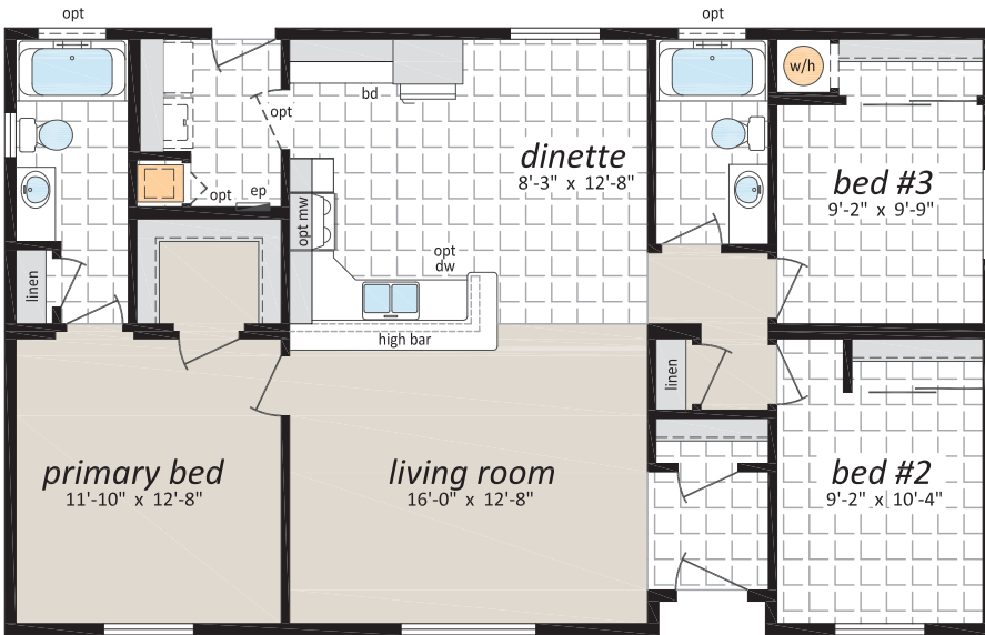
Galiano, 27GL4402 27' x 44' | 1,188 sq. ft. 3 Beds | 2 Baths
