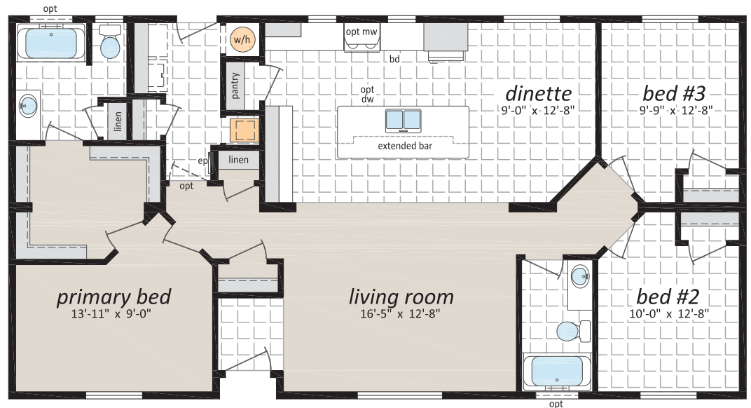
Kelowna, 27GL5201 27' x 52' | 1,404 sq. ft. 3 Beds | 2 Baths
