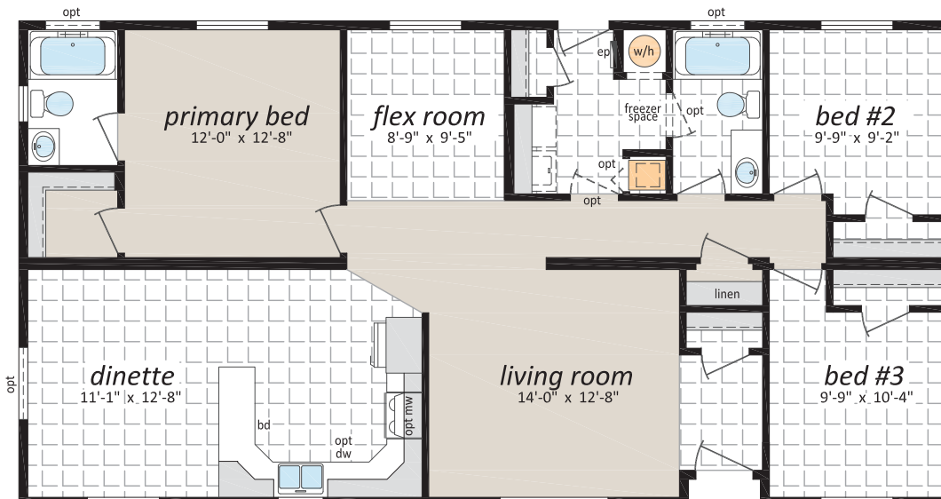
Saltspring, 27GL5202 27' x 52' | 1,404 sq. ft. 3 Beds | 2 Baths | Flex Room
